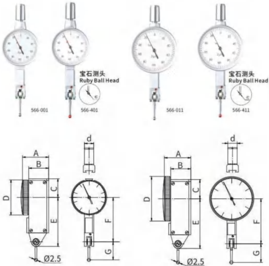
杠杆千分表Micron Dial Test Indicator 大表盘杠杆千分表Large Micron Dial Test Indicator
