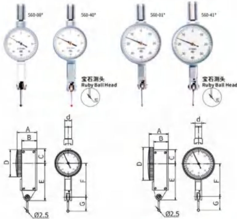
杠杆百分表 Dial Test Indicator
