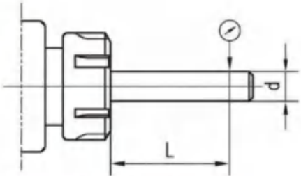
精度检测Inspection of Accuracy
